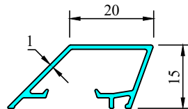
7545 W = 0.198 kg/m T = 1.0 mm
