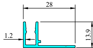
7598 W = 0.190 kg/m T = 1.2 mm
