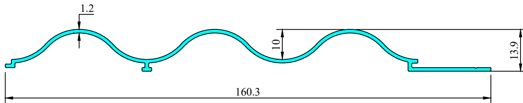
7600 W = 0.611 kg/m T = 1.2 mm
