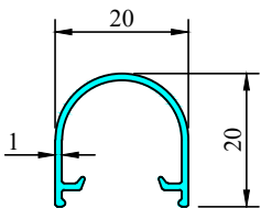
7593 W = 0.157 kg/m T = 1.0 mm
