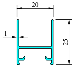
7594 W = 0.206 kg/m T = 1.0 mm
