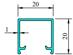
7329 W = 0.179 kg/m T = 1.0 mm
