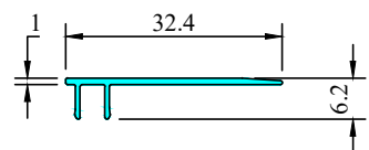
7599 W = 0.103 kg/m T = 1.0 mm
