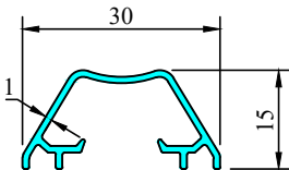
7597 W = 0.183 kg/m T = 1.0 mm
