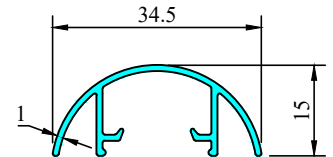
7596 W = 0.213 kg/m T = 1.0 mm
