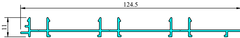
7328 W = 0.538 kg/m T = 1.0 mm
