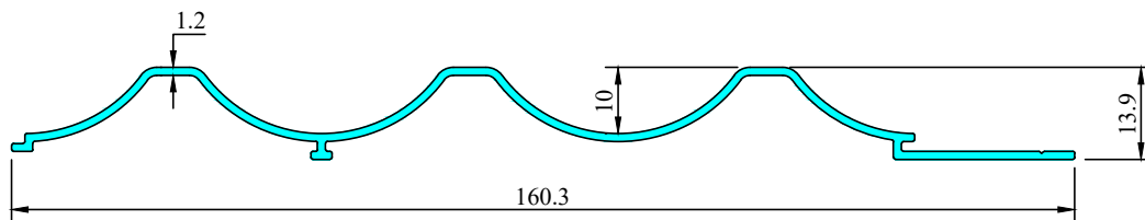
7601 W = 0.617 kg/m T = 1.2 mm
