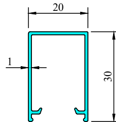
7595 W = 0.233 kg/m T = 1.0 mm
